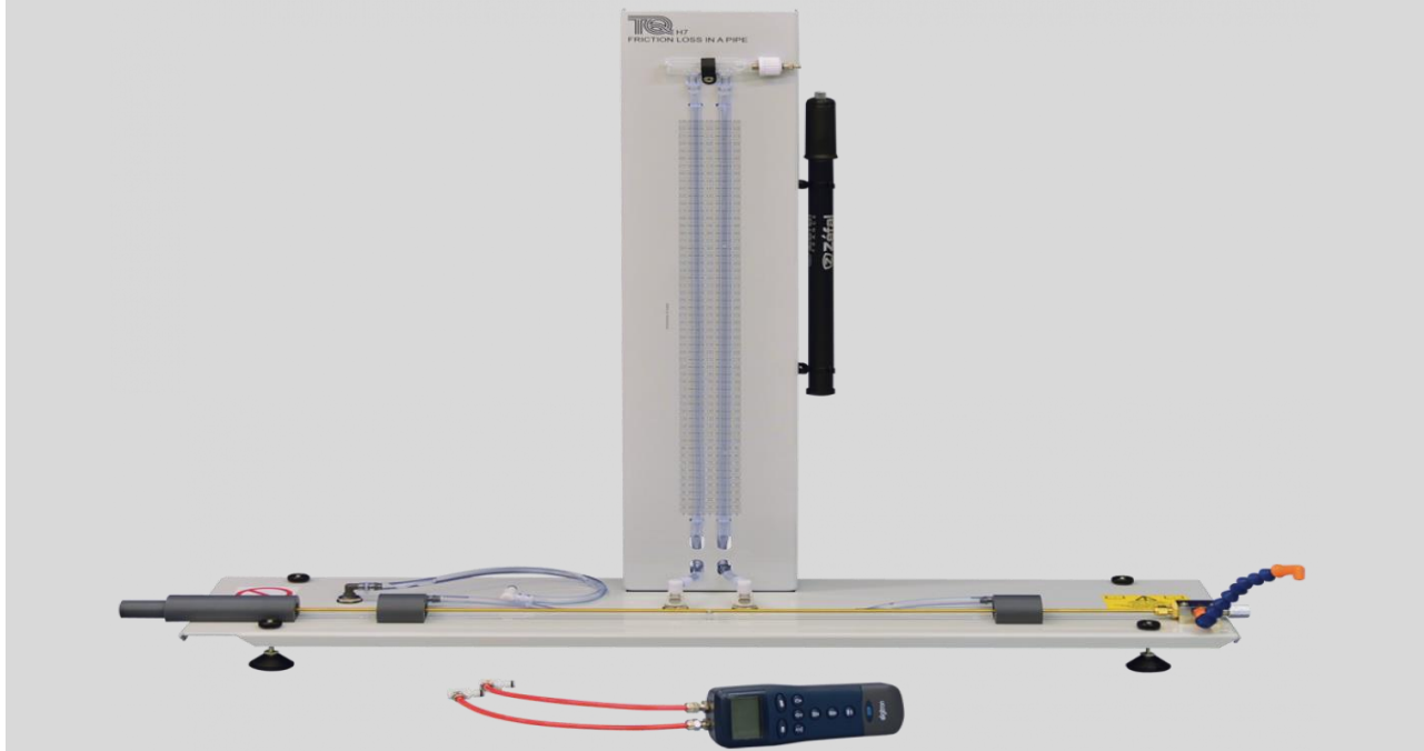
Friction loss in a pipe (TecQuipment)
