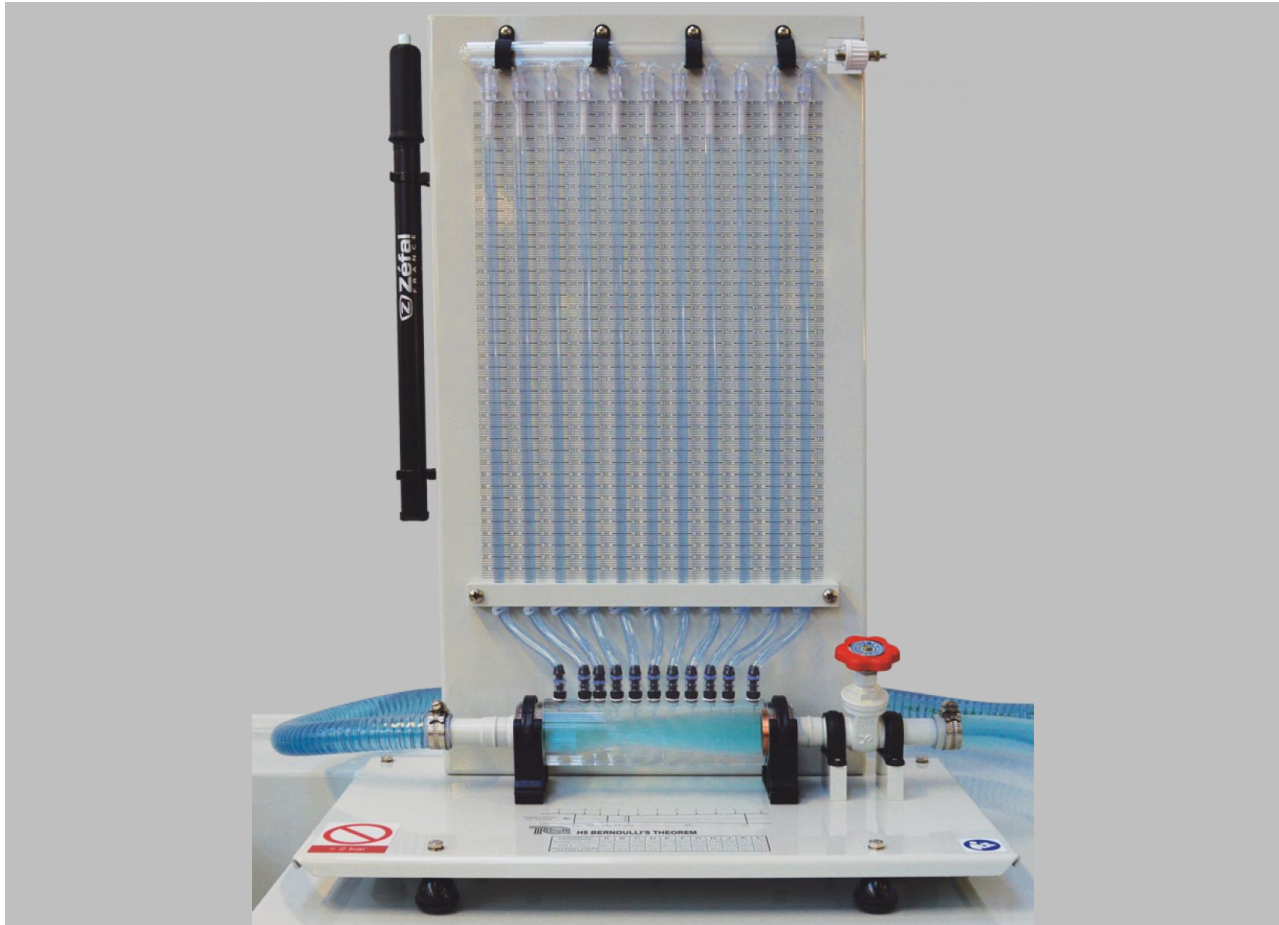
Bernoulli;s Theorem (TecQuipment)
